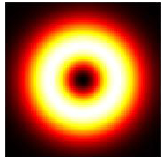
STED-Puls
