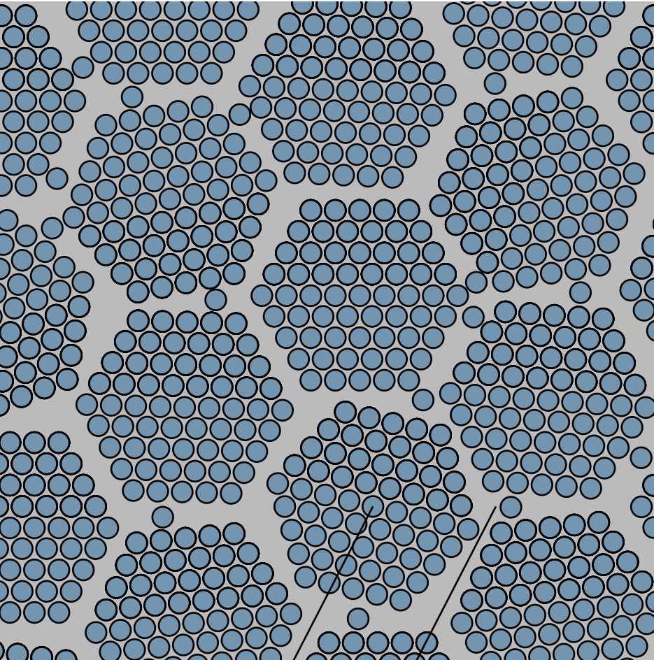
kristallines Metall
